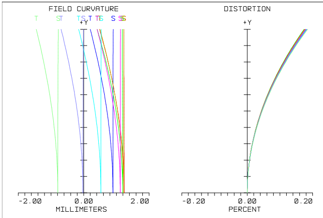
FIELD CURVATURE / DISTORTION MON MAR 8 2010 MAXIMUM FIELD IS 0.587 DEGREES WAVELENGTHS: 1.700 0.900 1.100 1.300 1.500 1.900 2.100 2.300 HORUS-D01.L05. 900-2300.ZMX CONFIGURATION 1 OF 2
