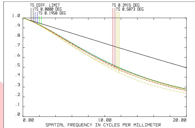
POLYCHROMATIC DIFFRACTION MTF MON MAR 8 2010 DATA FOR 1.7000 TO 2.3000 μm. SURFACE: IMAGE HORUS-D01.L05. 1700-2300.ZMX CONFIGURATION 1 OF 2
