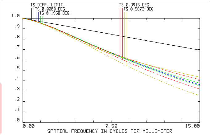
POLYCHROMATIC DIFFRACTION MTF MON MAR 8 2010 DATA FOR 0.9000 TO 2.3000 μm. SURFACE: IMAGE HORUS-D01.L05. 900-2300.ZMX CONFIGURATION 1 OF 2
